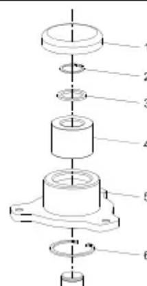
Fig.7 Balance wheel assy
